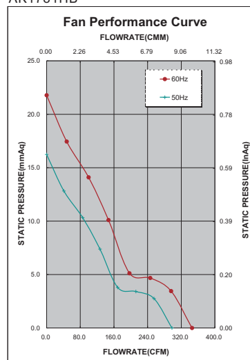
AK1781HB
