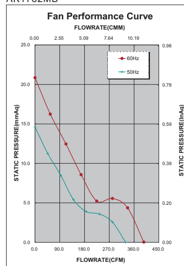
AK1782MB
